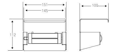
锁轴式卷纸架 (带平台) PAPER HOLDER WITH LOCK (WITH PLATFORM)
