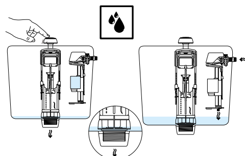
OPERATION MODE DUAL FLUSH
