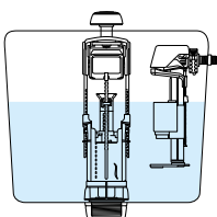
INLET VALVE IN CLOSED POSITION
