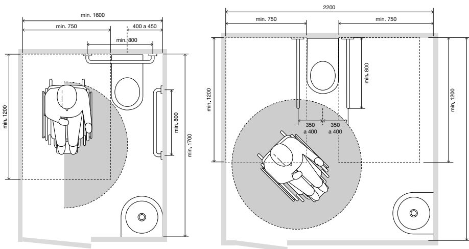
MINIMUM DIMENSIONS REQUIRED FOR THE INSTALLATION OF THE EASY MOVE WC
