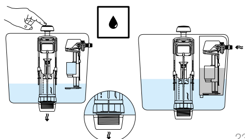
OPERATION MODE HALF FLUSH
