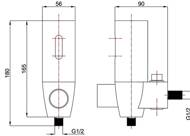
Product size: W56x D90x H165mm
