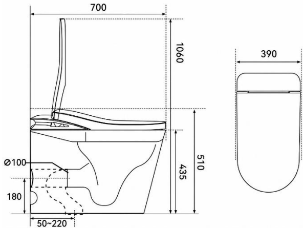
Product size : W390x D700x H510mm
