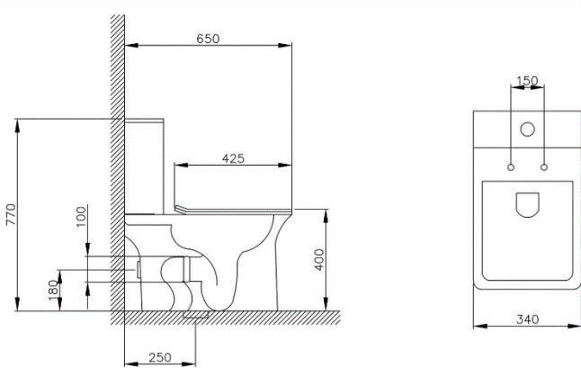
Product size : W340x D650x H770mm
