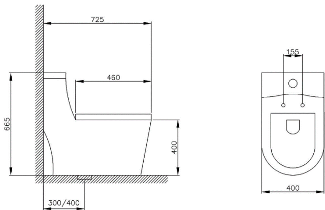
Product size : W400x D725x H665mm
